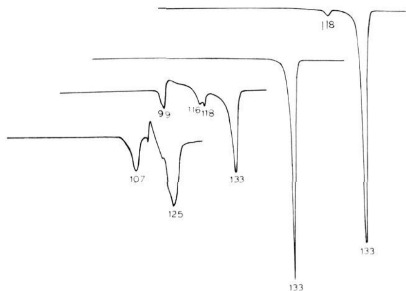
Figure 2. Differential scanning calorimeter traces showing the progress of the reaction of quinhydrone formation by grinding together 8c and 9 . (a) lower curve) An unground mixture of the starting materials, (b, lower-middle curve) reaction at an intermediate stage—note the endotherm at 133 °C due to the complex that has been formed, (c, upper-middle curve) completed reaction, and (d, upper curve) an artificial mixture of the quinhydrone complex to which has been added 1% of the naphthoquinone in order to test the sensitivity of the method.
